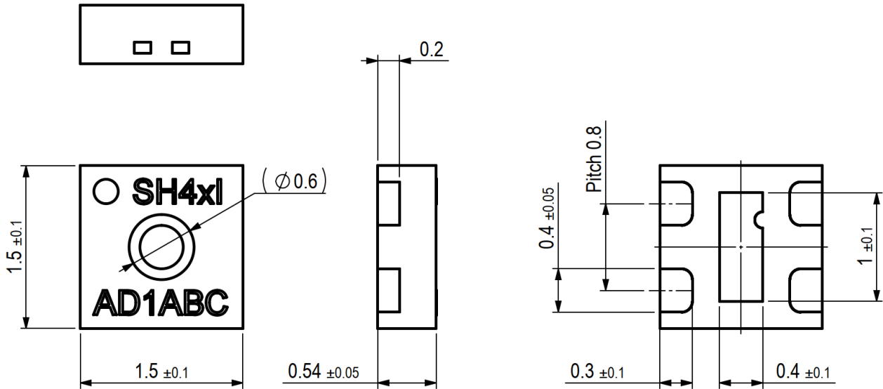
Figure 9. Dimensional drawing of SHT4xI-Digital including package tolerances (units mm).
