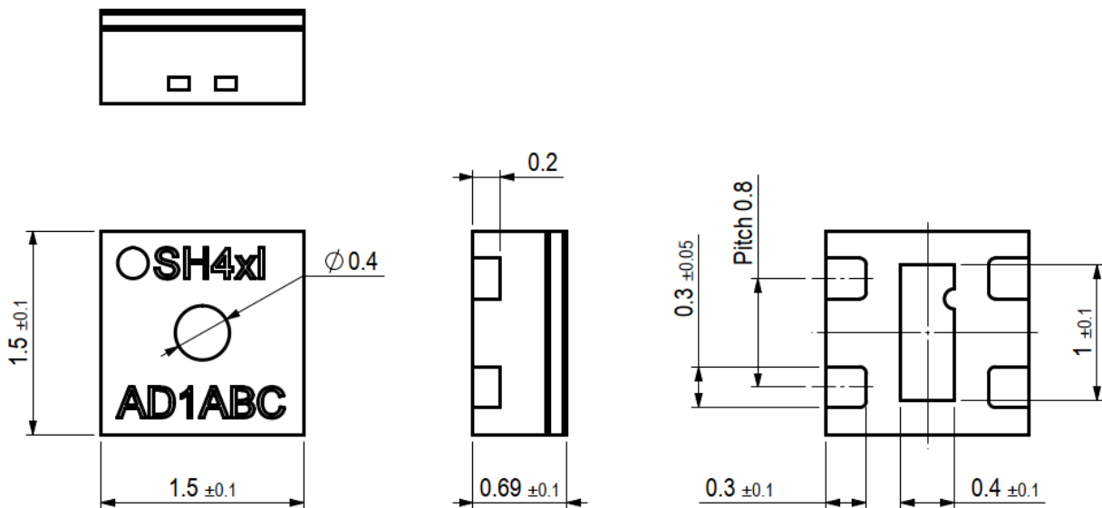
Figure 10. Dimensional drawing of SHT4xI-Digital with filter membrane including package tolerances (units mm)
