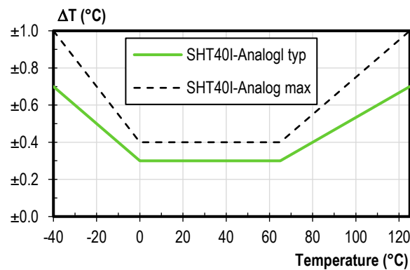
Figure 3. SHT40I analog typical and maximal temperature accuracy.
